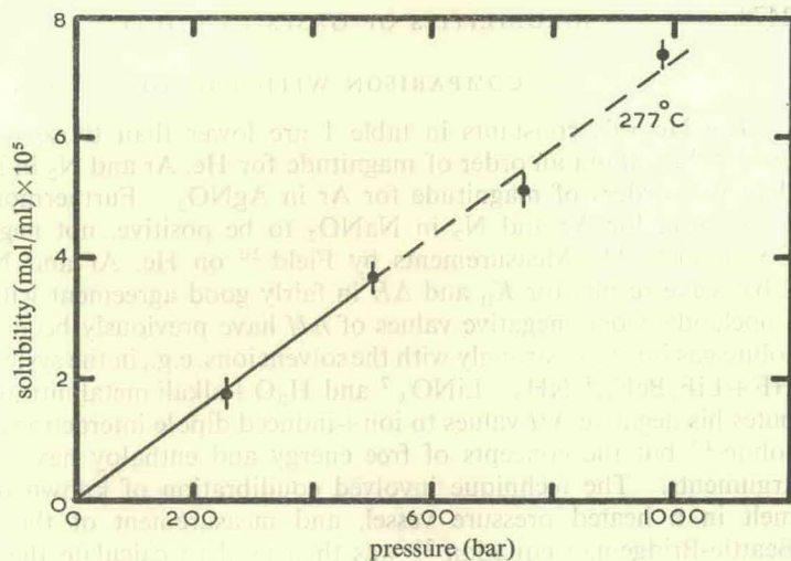
FIG. 5(c).—Solubility isotherm for the system N_2 + LiNO_3 .
