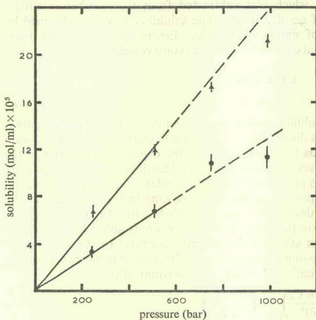
FIG. 6.—Solubility isotherms for the system Ar + RbNO_3 . ▲, 440°C; ●, 331°C.
